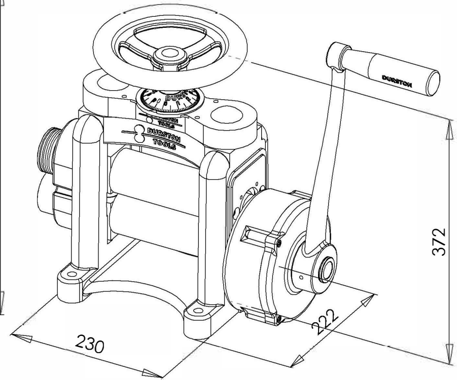
DRM F150RE Rolling Mill SKU: 1032 Dimensions is MM
