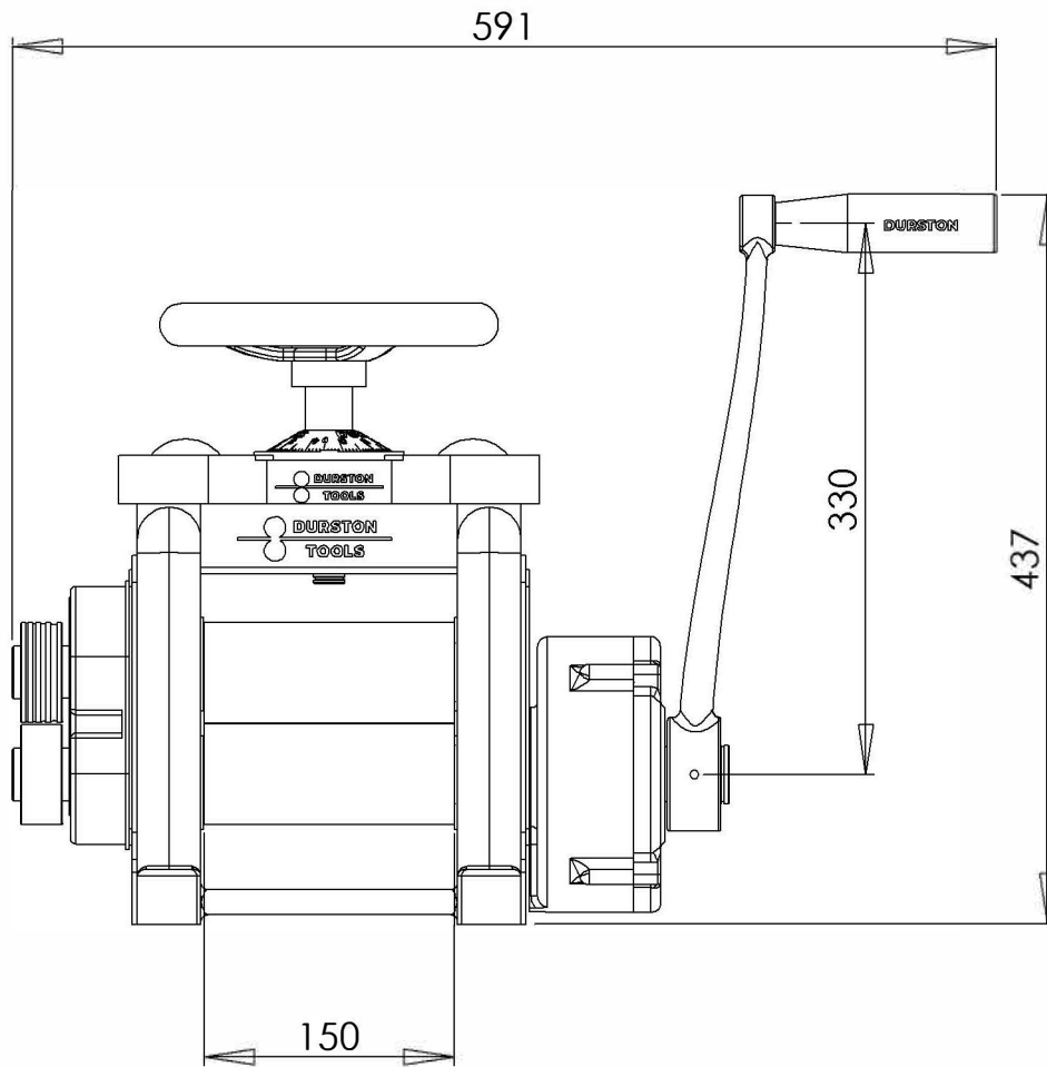
DRM F150RE Rolling Mill SKU: 1032 Dimensions is MM
